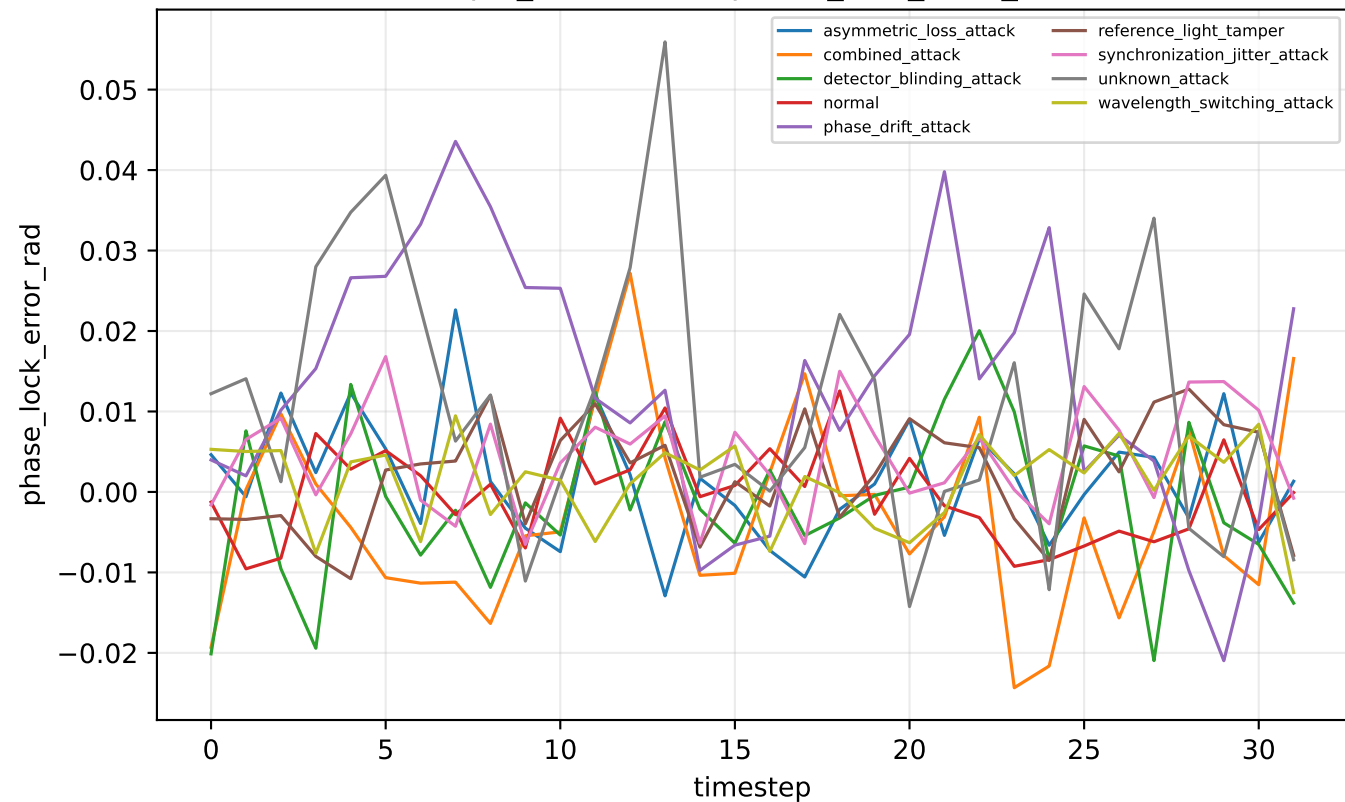
tfqkd_unknown — phase_lock_error_rad
