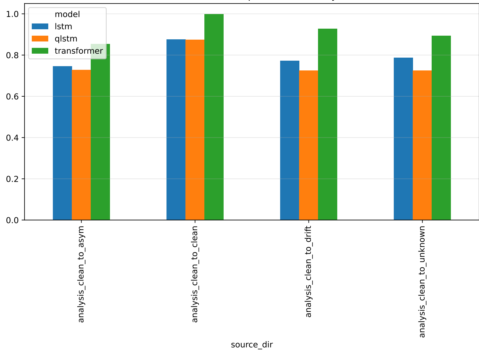
Cross-domain supervised accuracy
