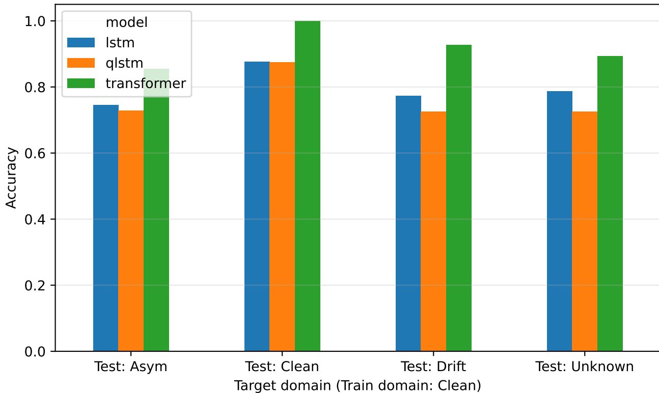
Cross-domain supervised accuracy
