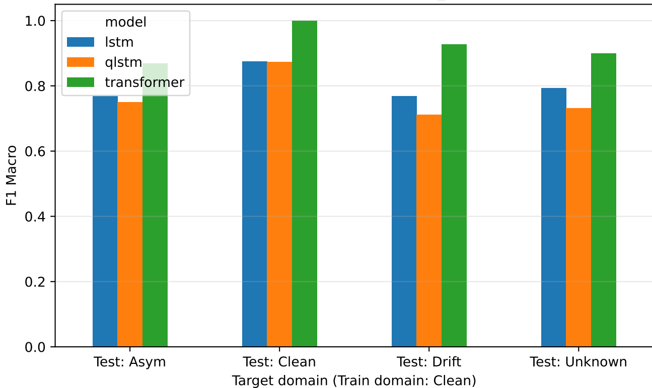
Cross-domain supervised f1_macro
