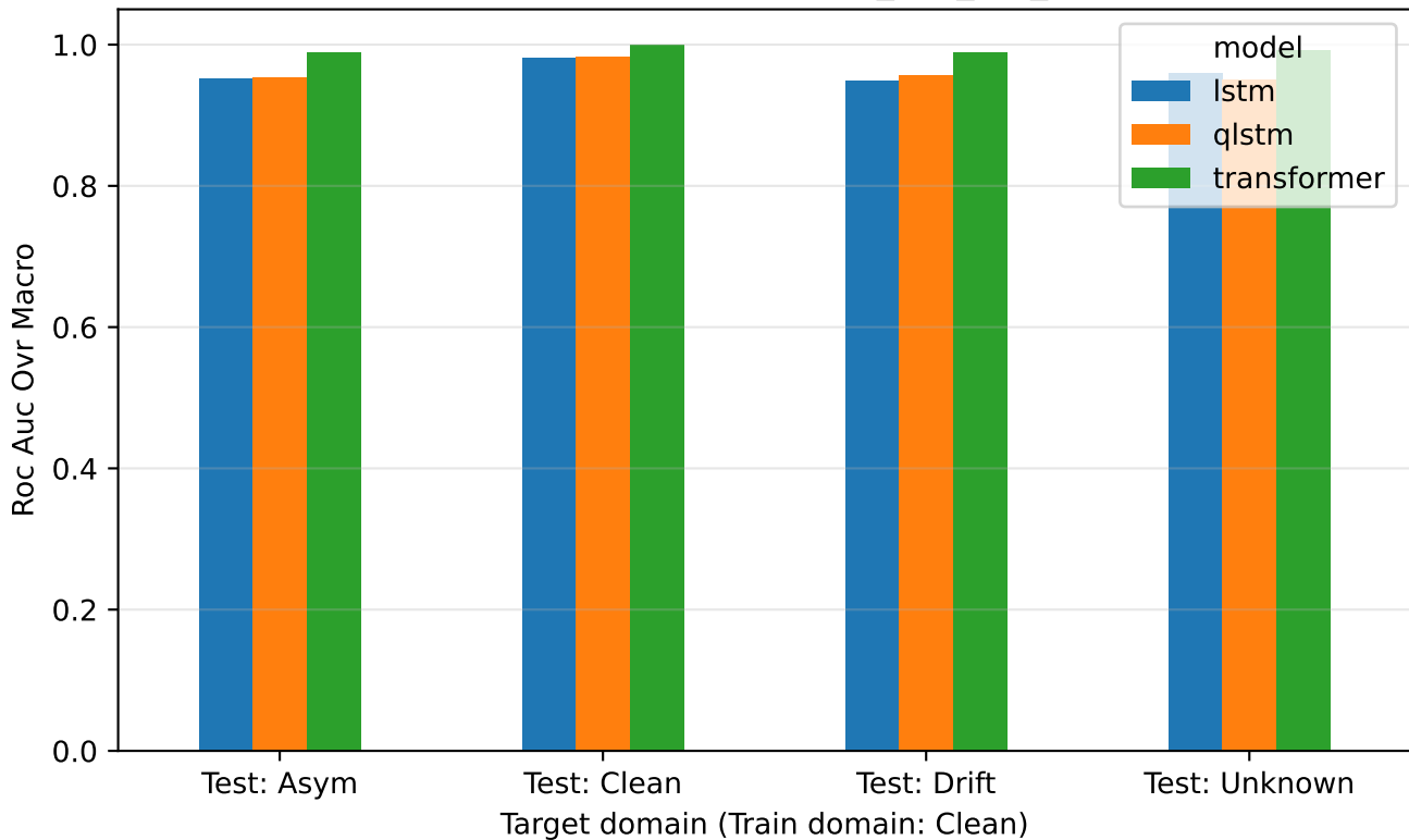
Cross-domain supervised roc_auc_ovr_macro
