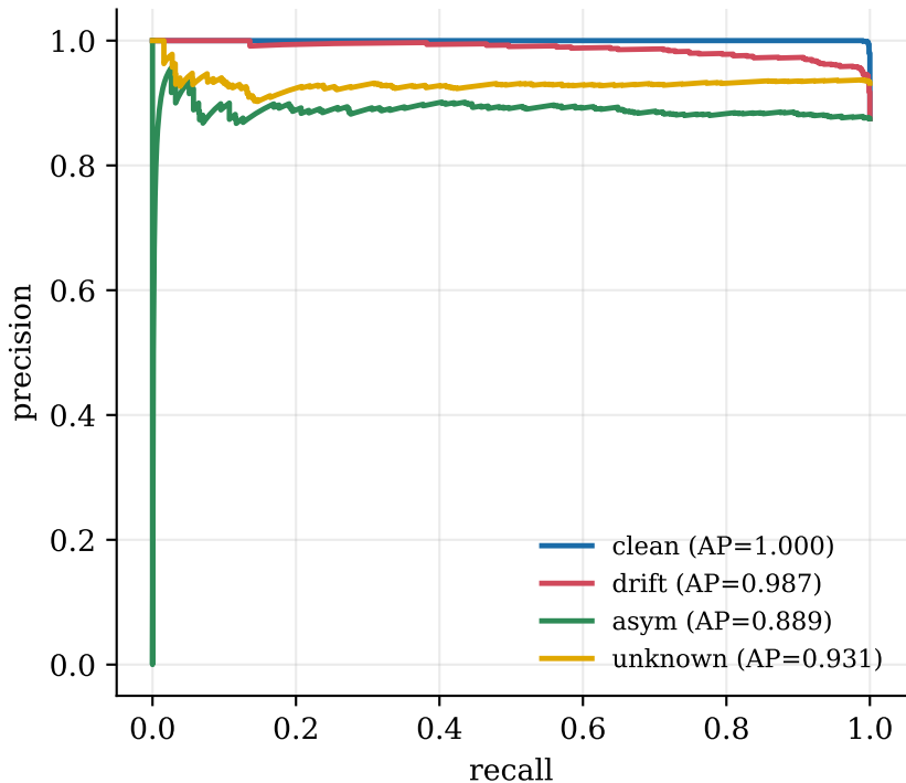
Anomaly precision-recall
