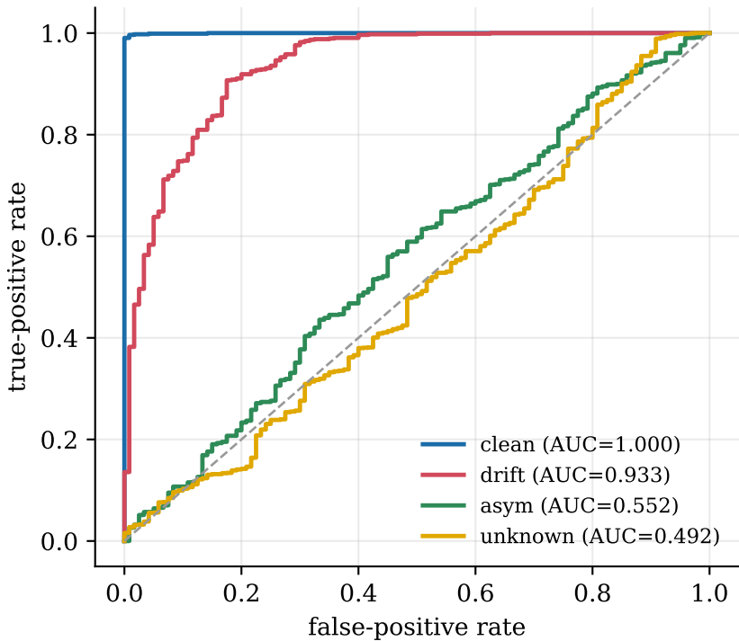
Anomaly ROC
