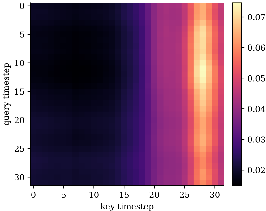
Transformer attention (last layer)
