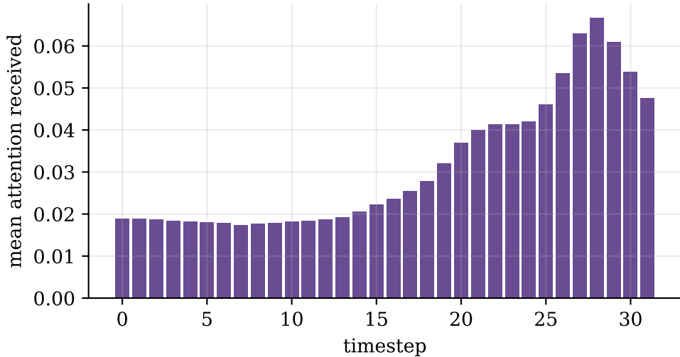
Temporal attention concentration
