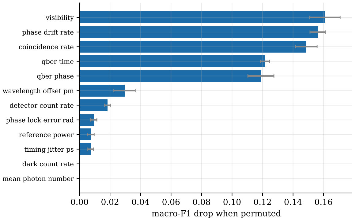
Channel importance (permutation)
