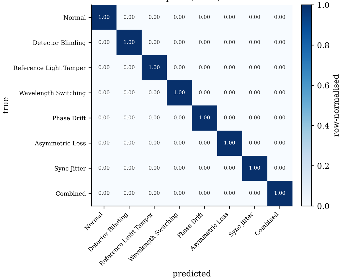
qlstm (clean)
