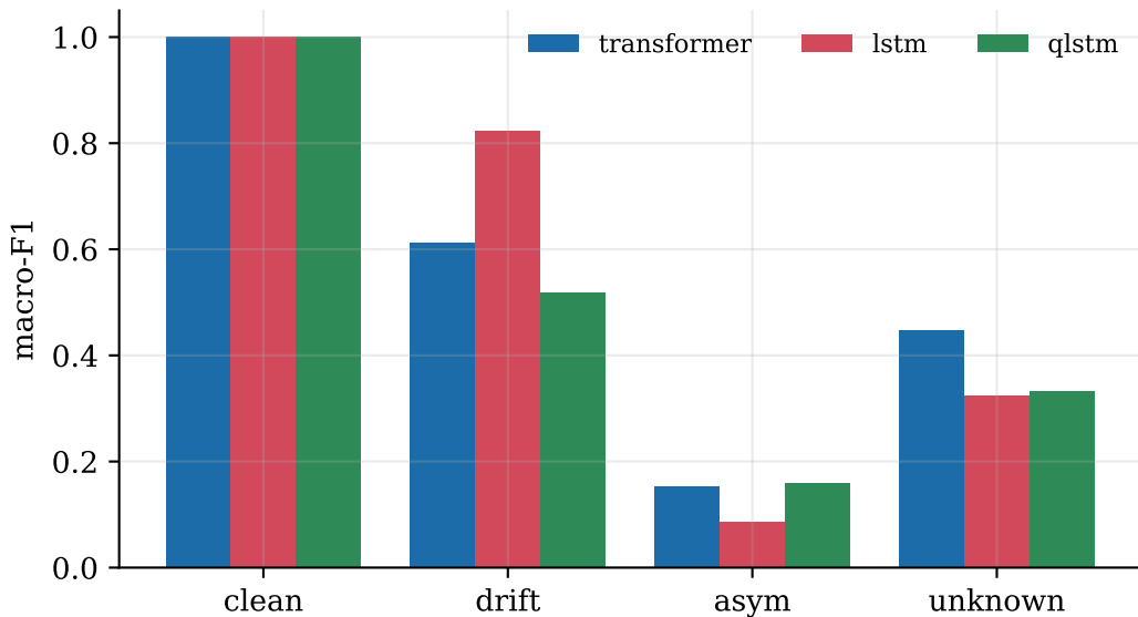
macro-F1 across domains
