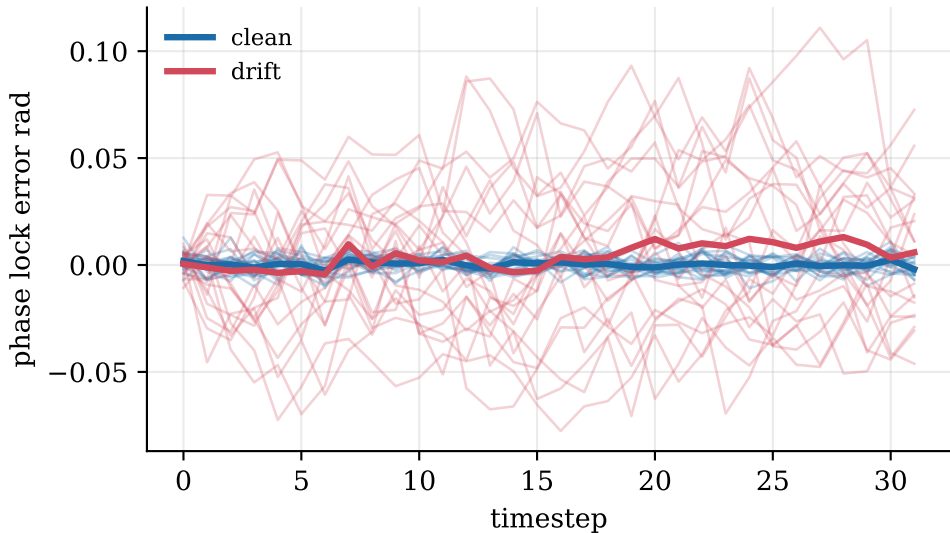
phase lock error rad: clean vs drift
