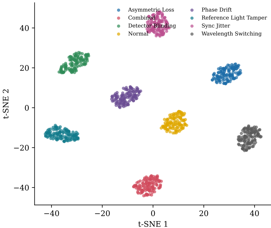
Latent embedding (t-SNE)
