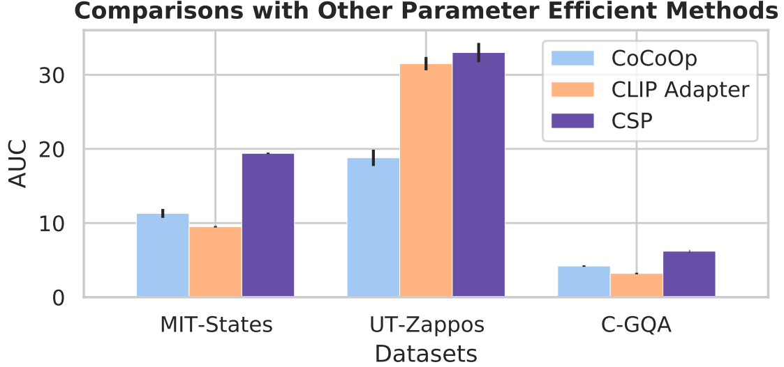
Figure 3.6: Closed-world results on MIT-States, UT-Zappos, and C-GQA comparing CoCoOp (Appendix 3.9), CLIP adapters (Appendix 3.10), and CSP. We report the average AUC on 5 random seeds.
