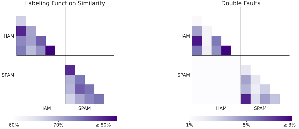
Figure 5.2: Visualization of the similarity matrix for labeling functions in the YouTube dataset compared with double faults, i.e., examples on which both labeling functions make a mistake.
