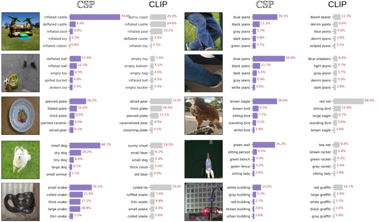
Figure 3.8: Additional qualitative comparison for image to text retrieval between CSP and CLIP on CGQA. Selected samples with concepts correctly identified and top-5 retrieval results by CSP are shown.
