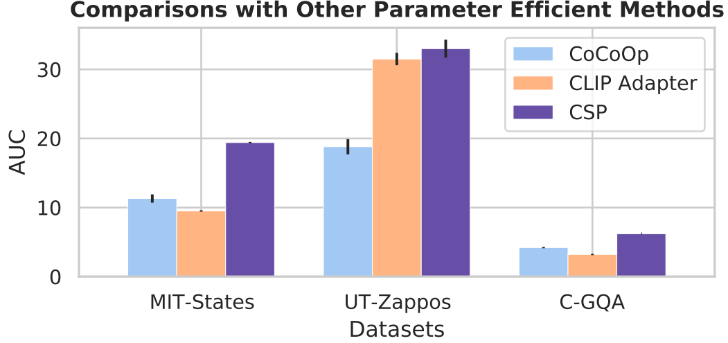
Figure 3.6: Closed-world results on MIT-States, UT-Zappos, and C-GQA comparing CoCoOp (Appendix 3.8), CLIP adapters (Appendix 3.9), and \mathcal{CSP} . We report the average AUC on 5 random seeds.
