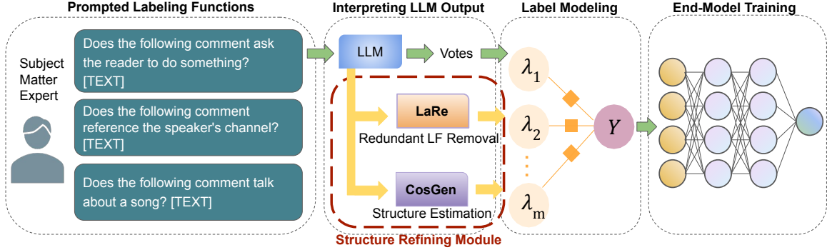
Figure 6.1: Prompted weak supervision workflow showing the Structure Refining Module as a plugin.
