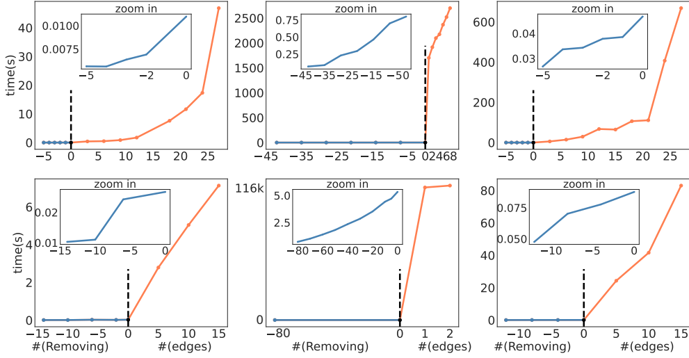
Figure 6.4: Label model running time for LaRe (left side of the dashed vertical line; plotted using blue) and CosGen (right side of dashed vertical line; plotted with orange). We zoom in the LaRe (blue plots) to better show the tendency in the subplots. From left to right columns are plots for Youtube, SMS and Spouse respectively. The first row describes experiments with original set of prompted LFs and the second row describes experiments with augmented LFs.
