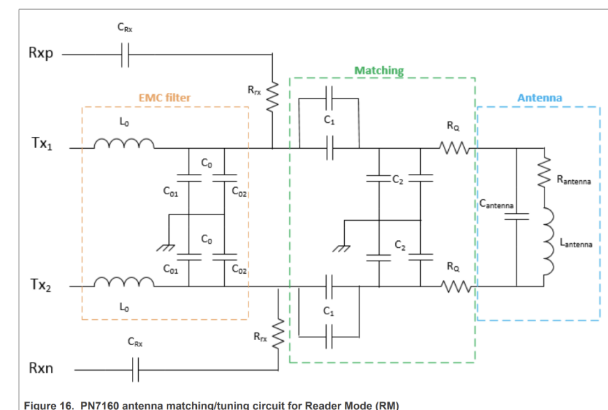
Figure 16. PN7160 antenna matching/tuning circuit for Reader Mode (RM)
