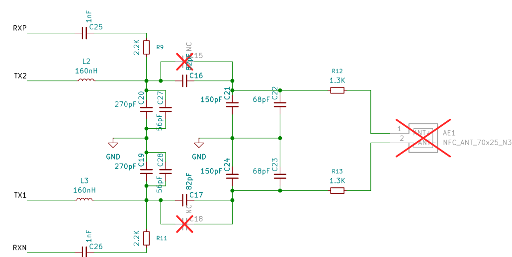
Figure 16. PN7160 antenna matching/tuning circuit for Reader Mode (RM)
