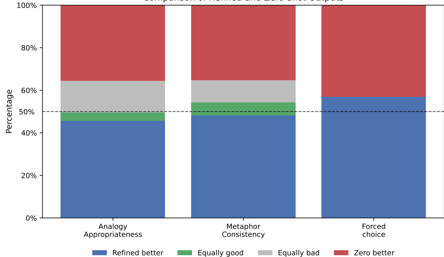
Comparison of Refined and Zero-shot Outputs
