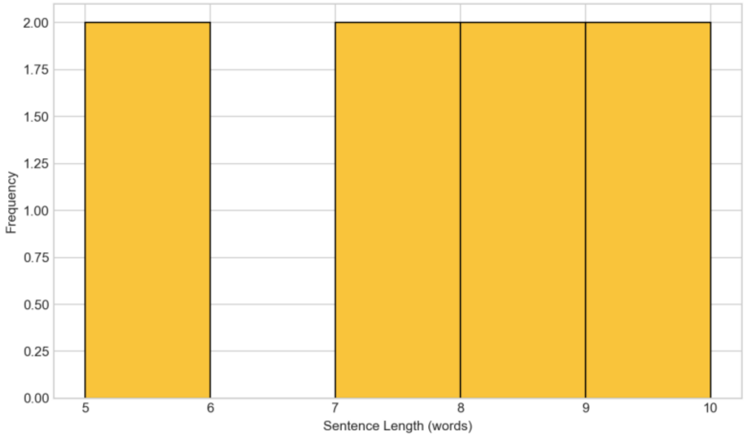
Sentence Length Distribution
