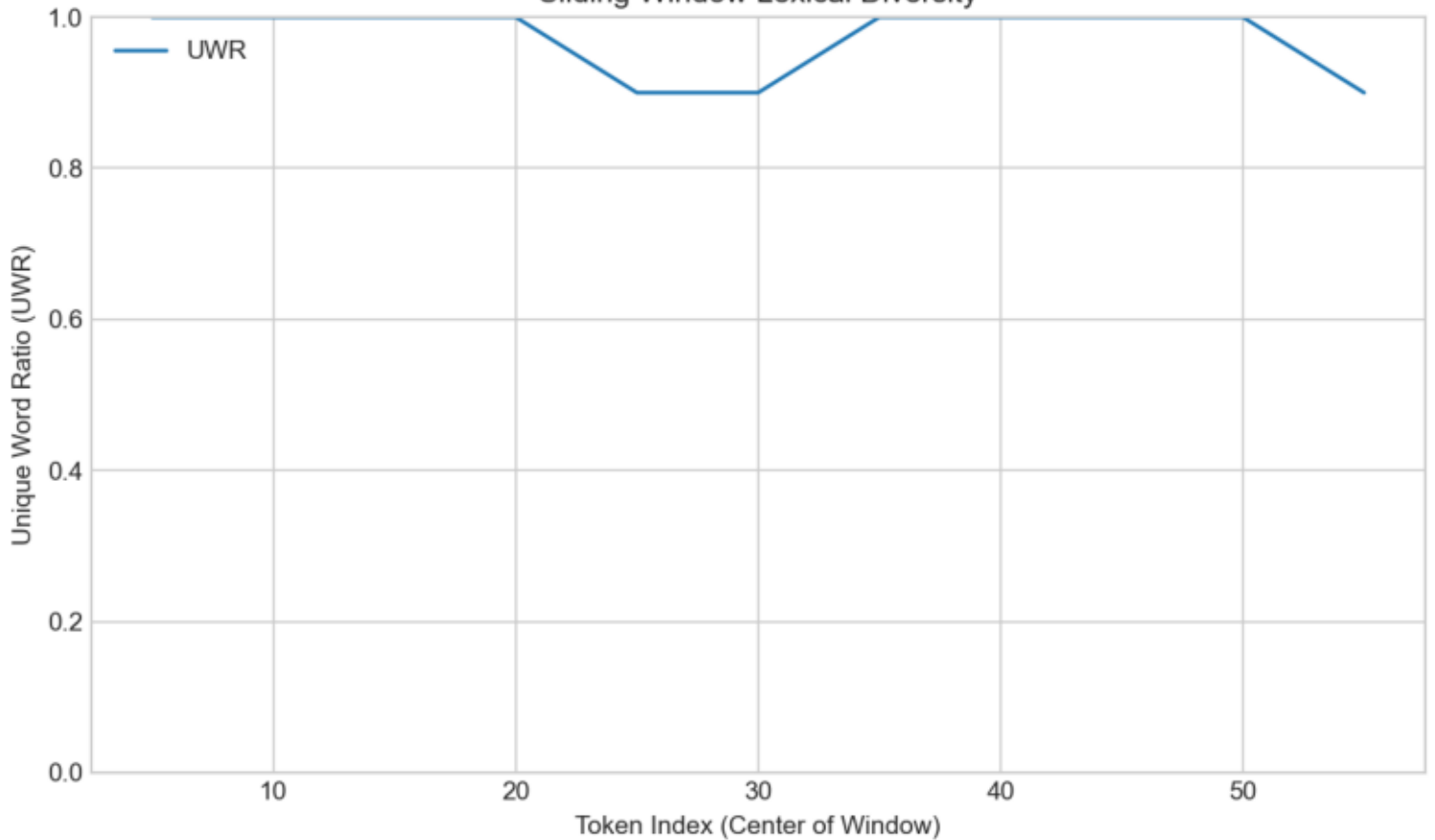
Sliding Window Lexical Diversity
