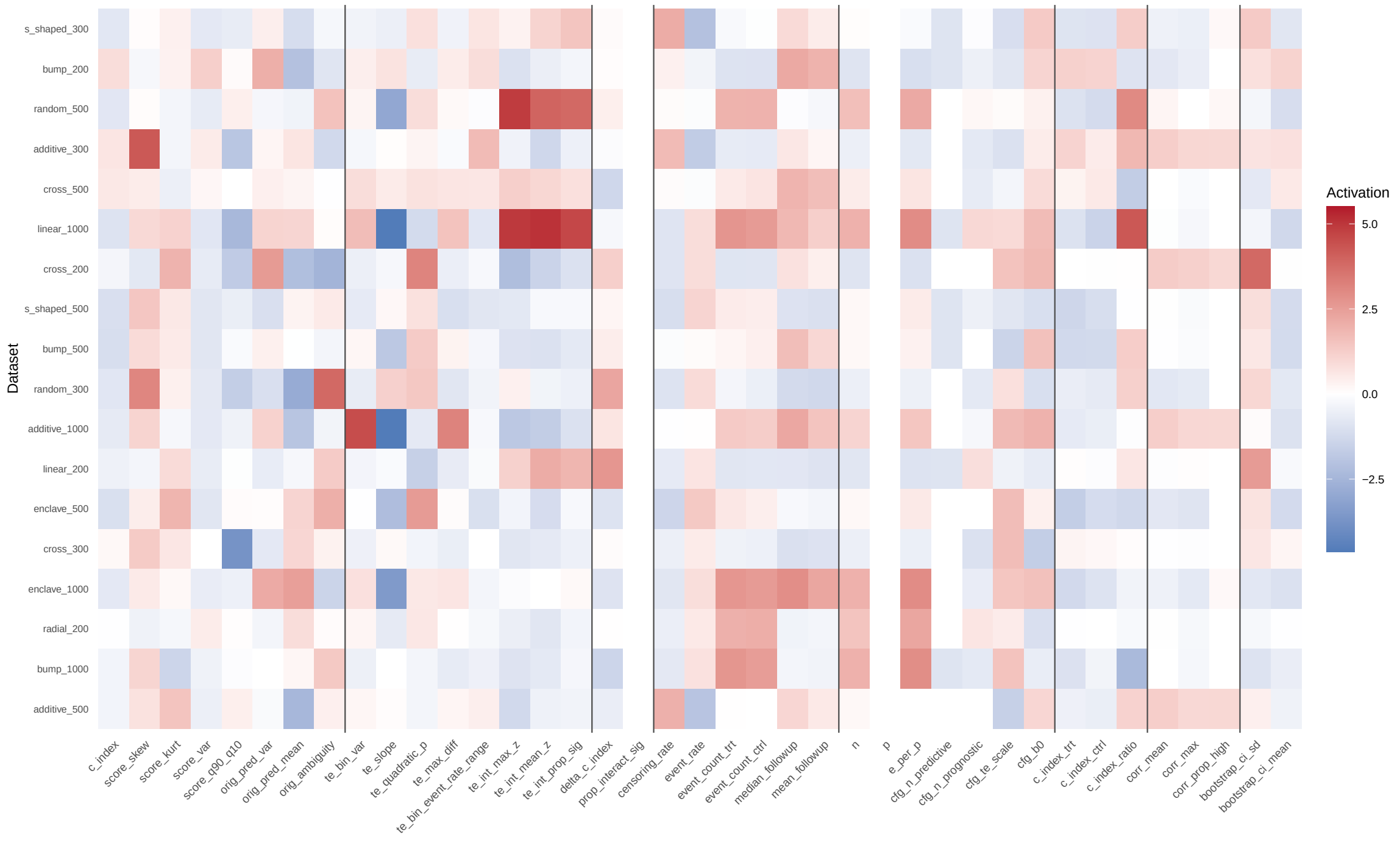
Gate RF: Per-Dataset Activation Map (Test Set)
