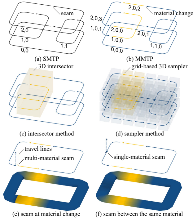
6 [a]–[d] A 3-layer minimal example showing the data structures and material assignment methods. Gaps between layers are exaggerated. [e], [f] Multi-material seam defect. Space between segments is added for display.
