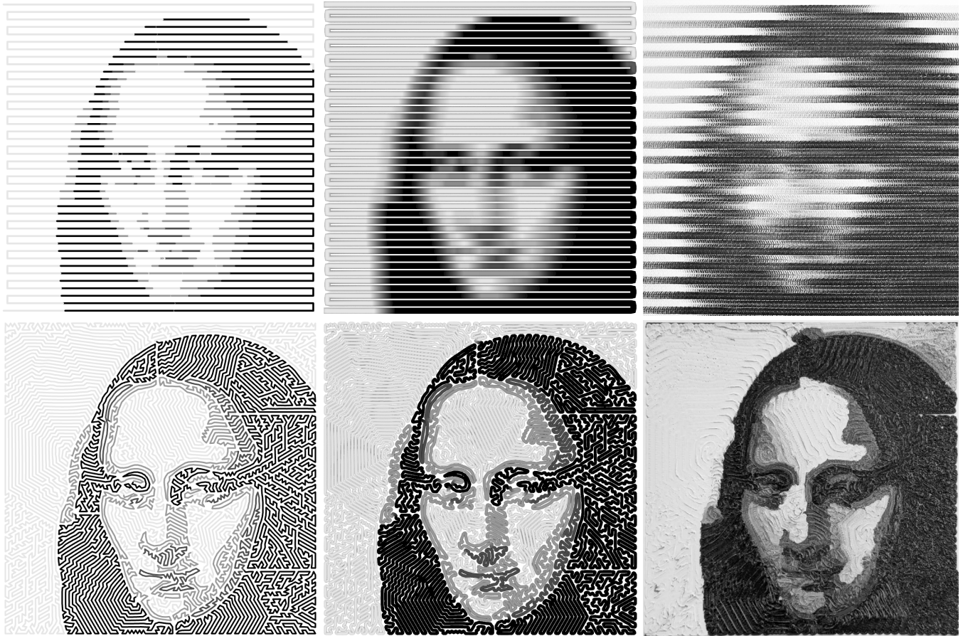
9 200 × 200 mm 2D gradient multi-material extrusion of a posterized image from the Mona Lisa . Top row: Soft-edge parallel filling. Bottom row: Hard-edge alpha complex filling. Left: Toolpath before transition adjustments. Middle: Visualization. Right: The finished prints.
