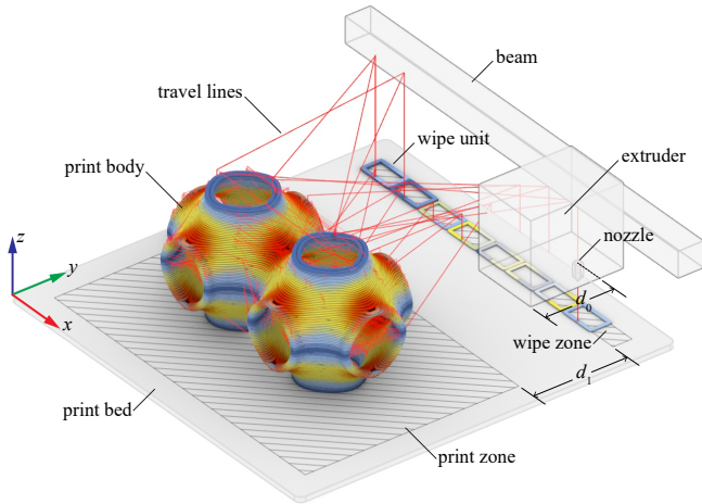
7 Print scheme of two cells of Schwartz P TPMS on a 300 x 300 mm print bed, showing the wipe units. This 90-layer print uses 8 wipe units. Compared with a traditional wiping tower [at least 1 unit per layer], it saves 1 - 8/90 = 91\% of the wiping material, 11% of the total material. Timewise, it still saves 13.8% of the traveling time despite the large clearance added between the print and wipe zones.
