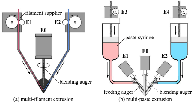
2 Schematic drawing of gradient multi-material extrusion systems with active mixing [E0] for (a) filament and (b) paste. Adapted from Teng et al. [2024] and Teng et al. [2025].
