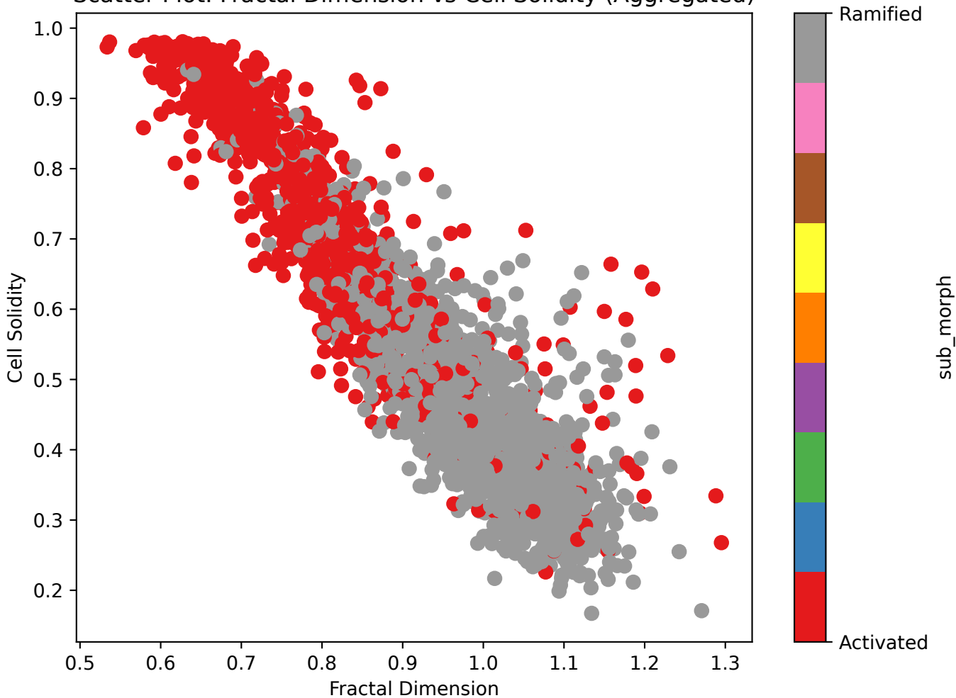
Scatter Plot: Fractal Dimension vs Cell Solidity (Aggregated)
