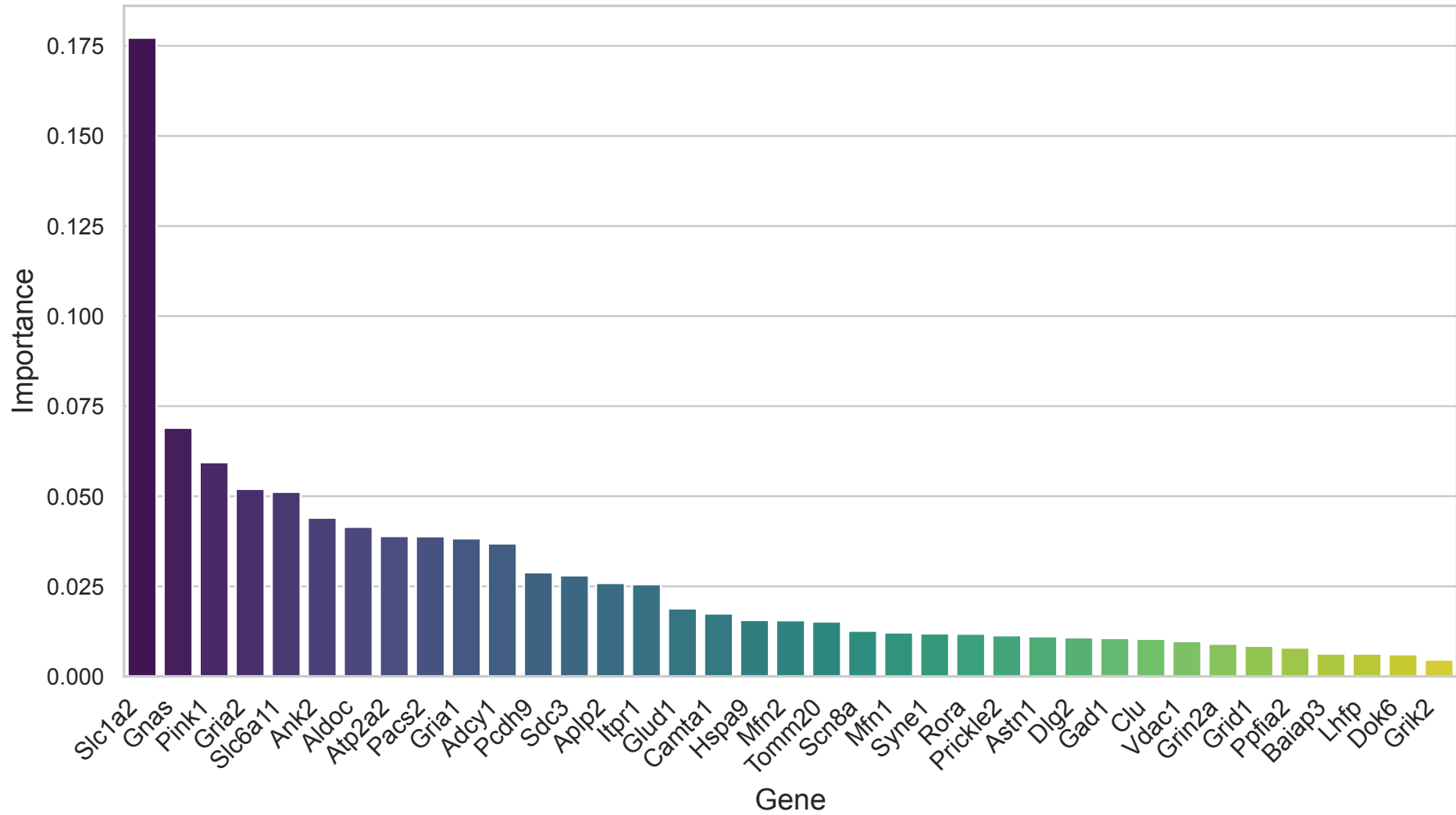
Gene Importance
