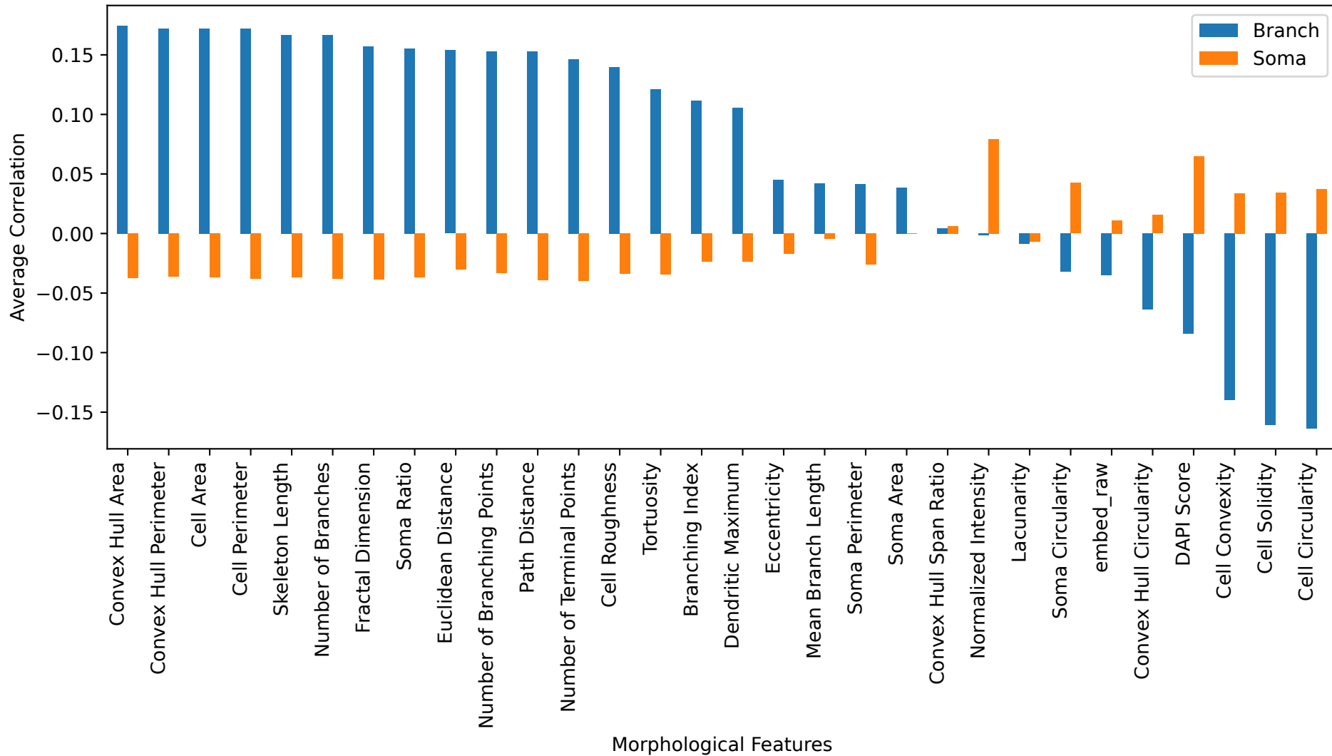
Average Spearman Correlation by Morphological Feature (Sorted by Branch Correlation)
