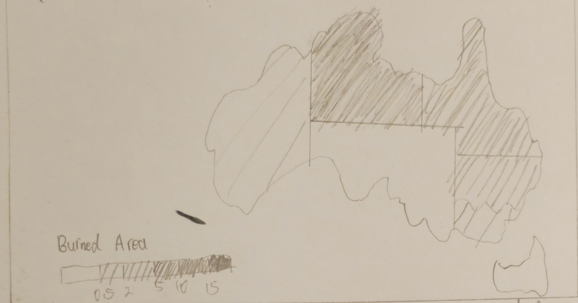
Forest Fire Extent Across Australia - Black Summer Season
