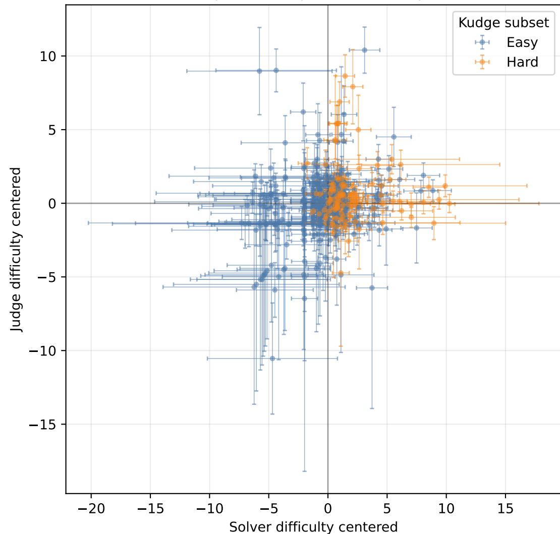
Solver vs Judge Difficulty ( \rho=0.219 , p=1.62e-05 )
