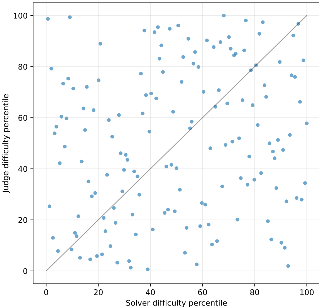
Solver vs Judge Difficulty Percentiles ( \rho=0.169 , p=0.0363 )
