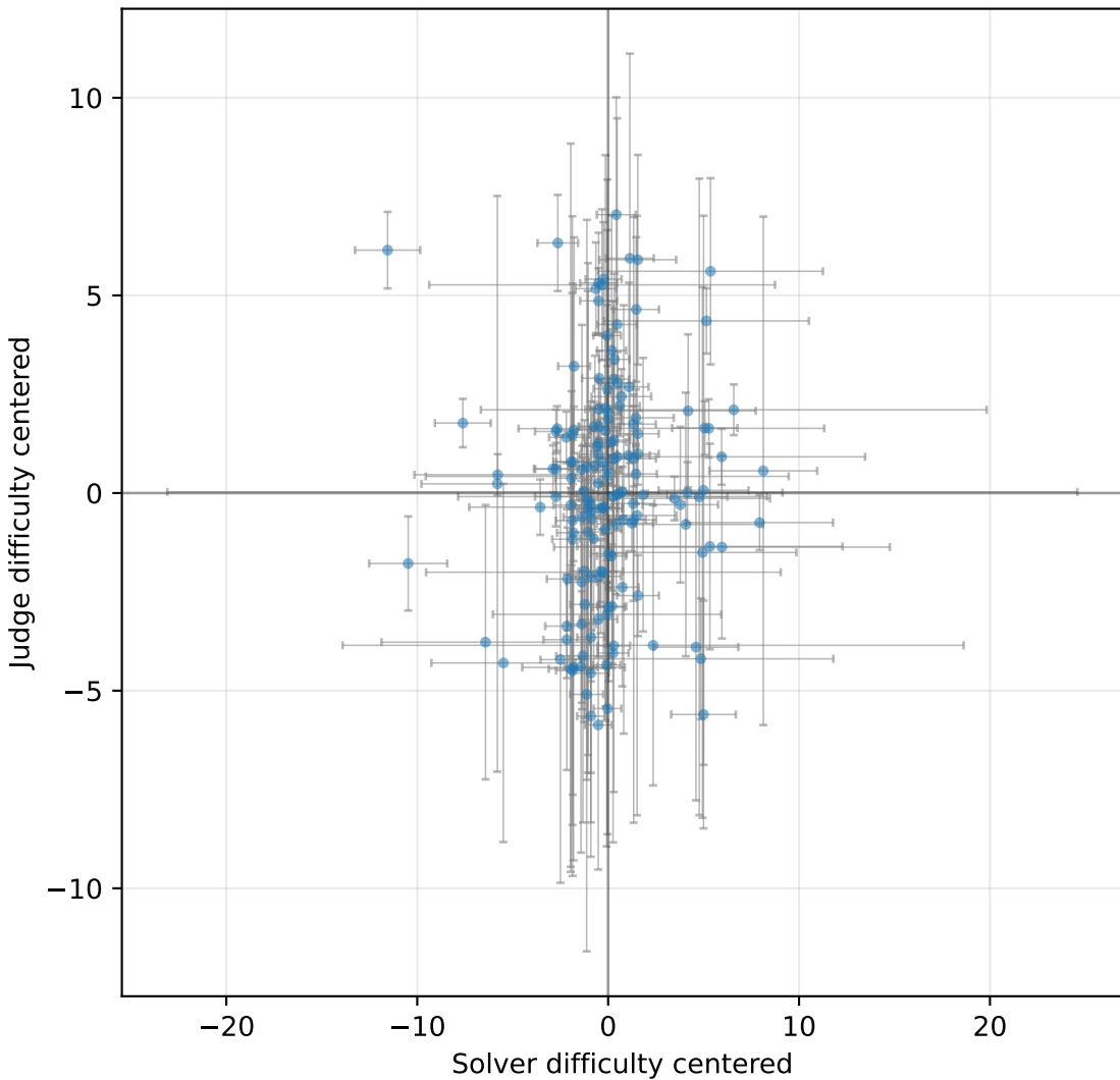
Solver vs Judge Difficulty ( \rho=0.169 , p=0.0363 )
