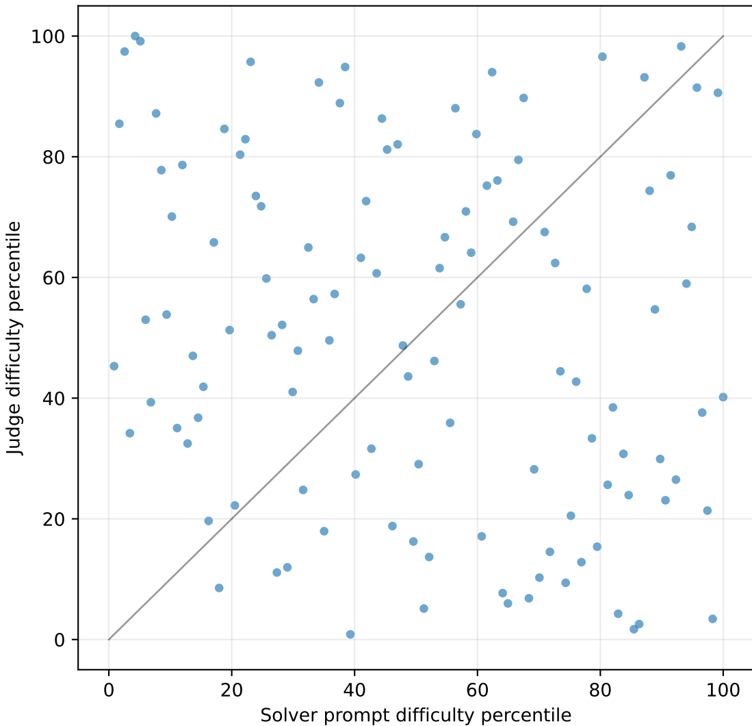
Solver vs Judge Difficulty Percentiles ( \rho=-0.197 , p=0.0332 )
