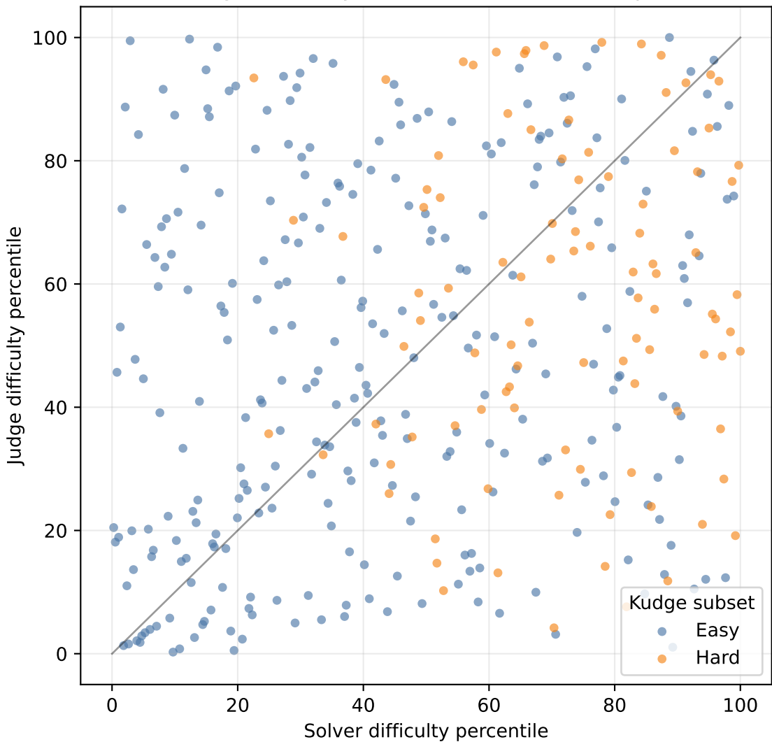
Solver vs Judge Difficulty Percentiles ( \rho=0.219 , p=1.62e-05 )
