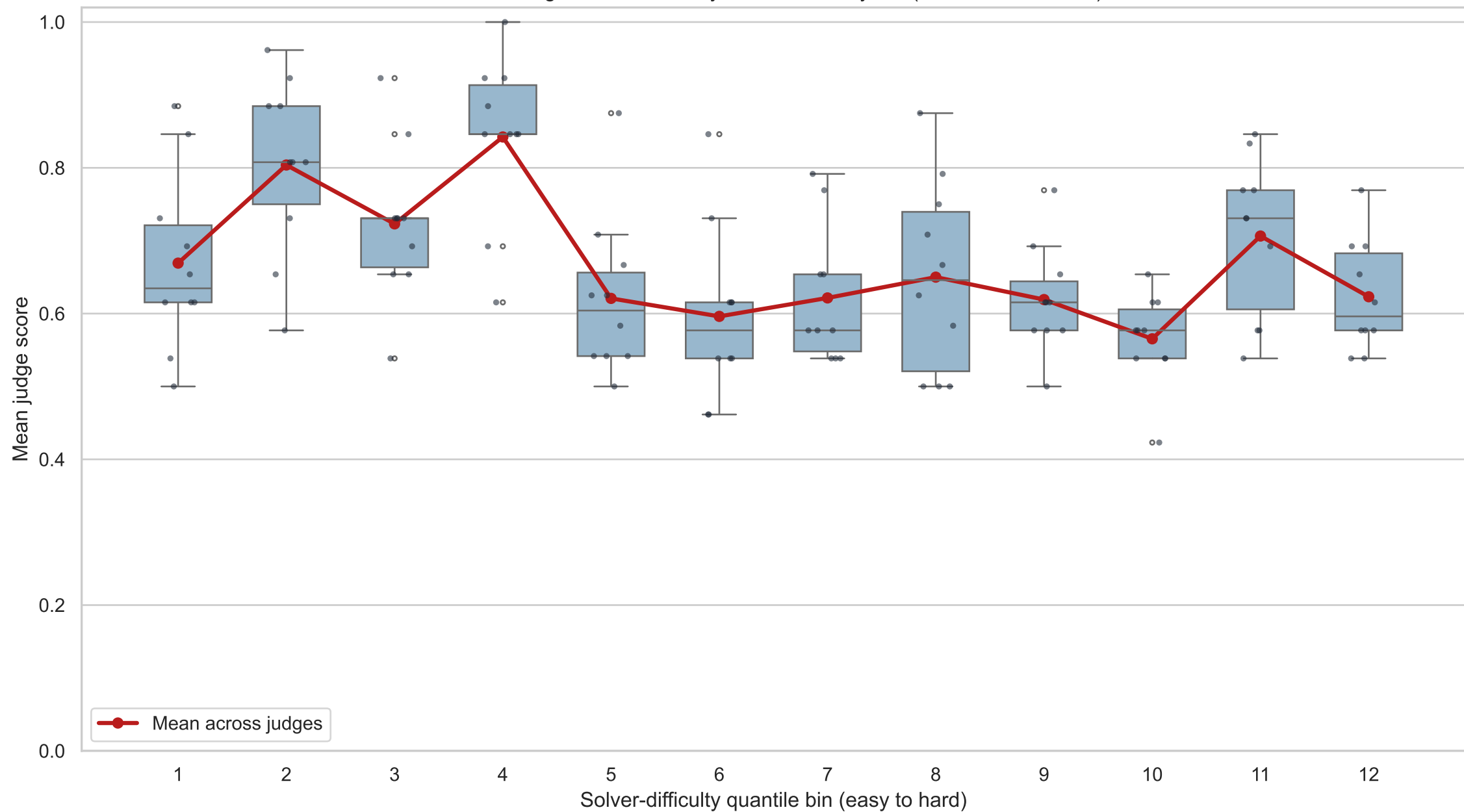
MMLU Judge Performance by Solver-Difficulty Bin (12 bins, K=1 solver)
