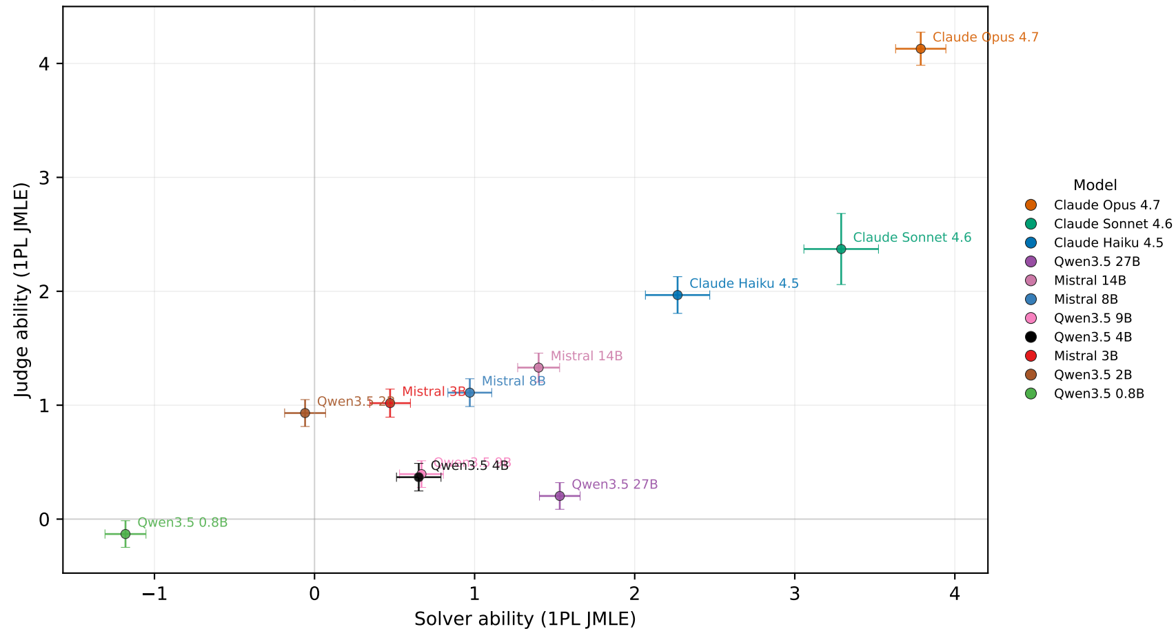
Kudge: Solver vs Judge IRT Ability Spearman rho=0.736, p=0.00976
