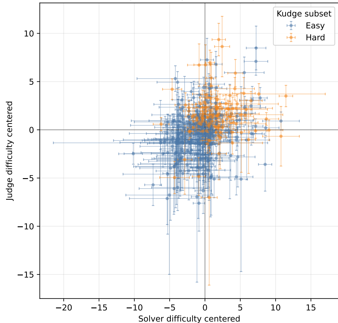
Solver vs Judge Difficulty ( \rho=0.341 , p=7.42e-12 )
