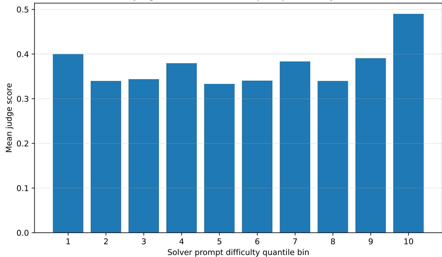
Mean judge score across solver prompt difficulty deciles
