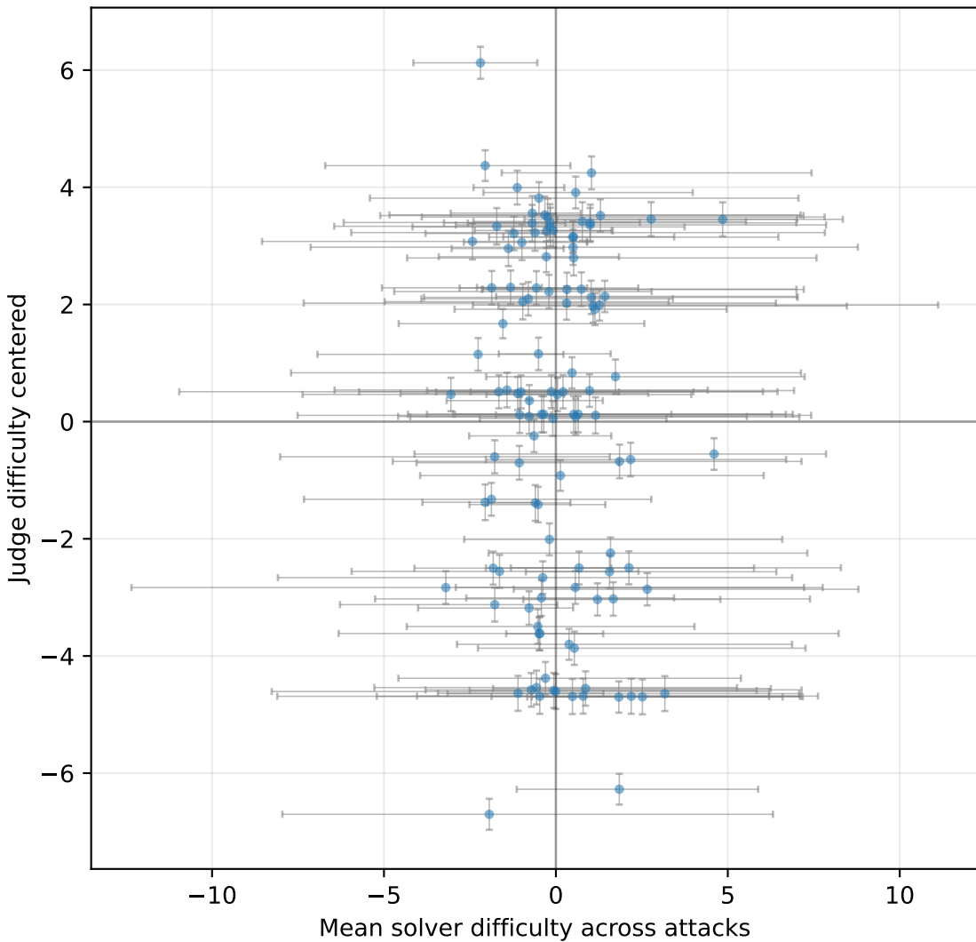
Solver vs Judge Difficulty ( \rho=-0.105 , p=0.261 )
