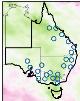
e) Aug IOD
