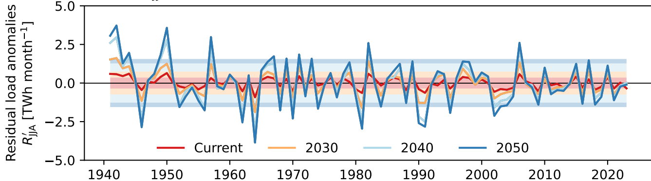
c) Winter (JJA) residual load anomalies and standard deviation 1940-2023
