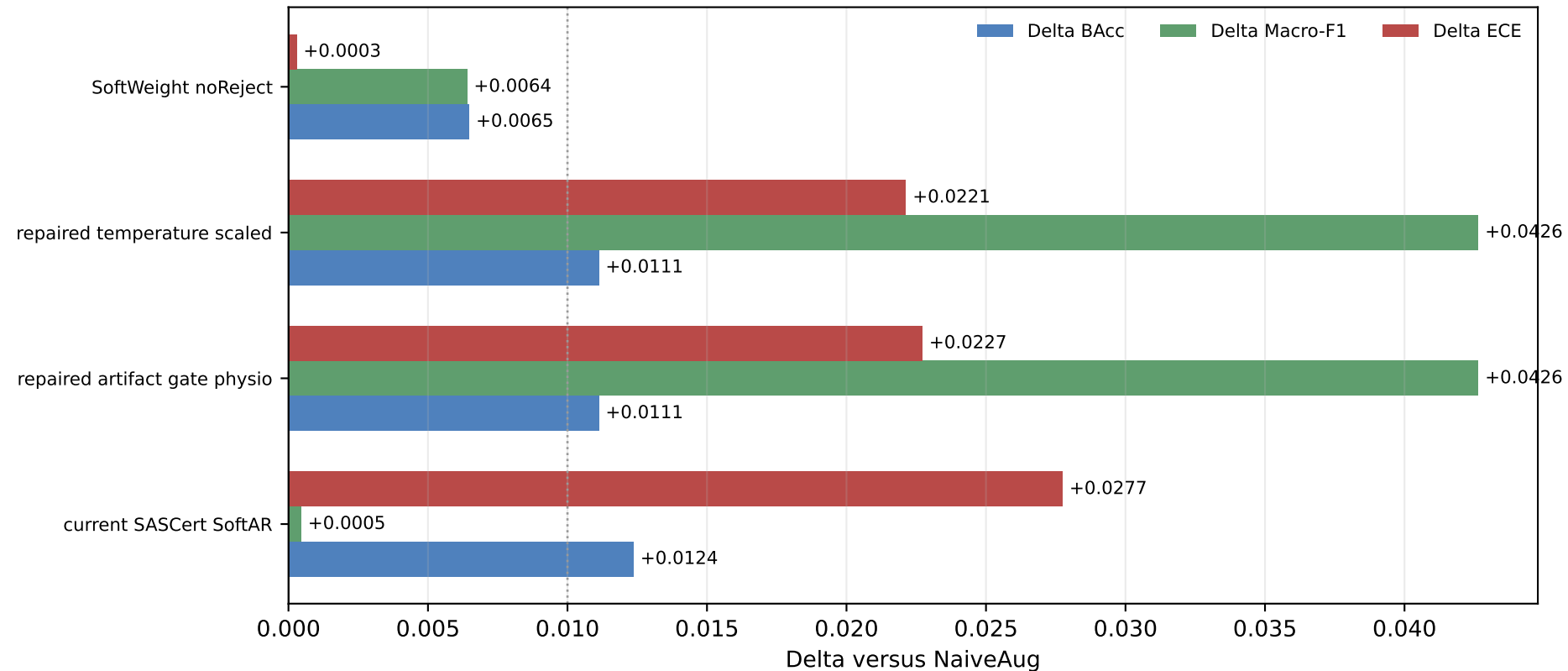
Training Policy Deltas and Non-Promotion Boundary
