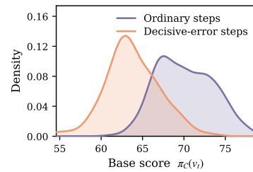
Figure 3: Base-score distribution on a CORRECT-ERROR test split. Decisive-error steps concentrate at smaller projection magnitudes than ordinary steps.
