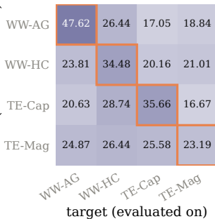
(c) Generalization
