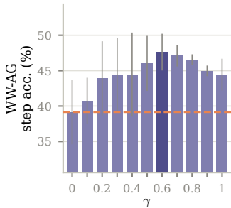
(a) Propagation strength \gamma
