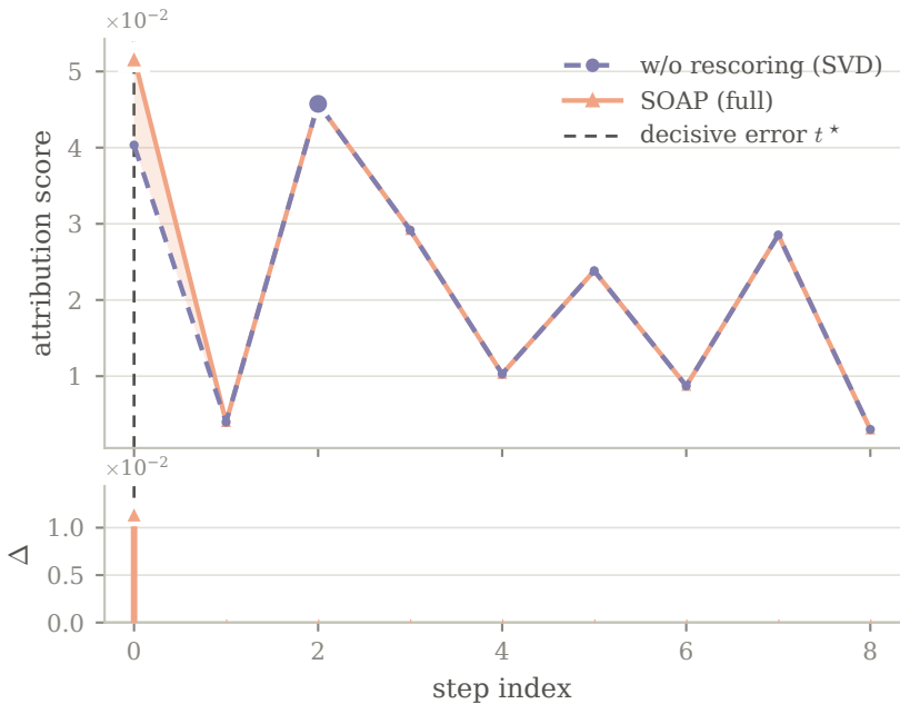
WW-AG · seed 6 · traj 43 (non-window seed)
