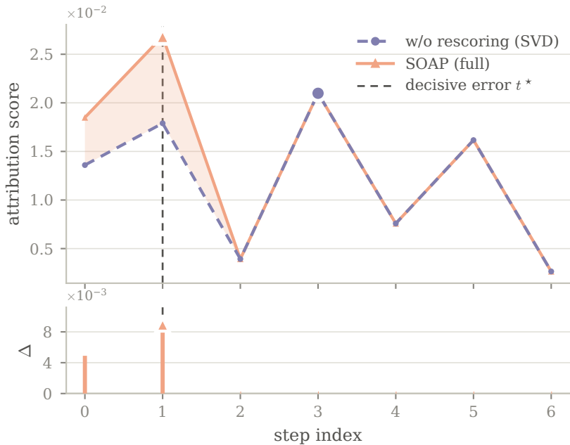
WW-AG · seed 7 · traj 121 (non-window seed)
