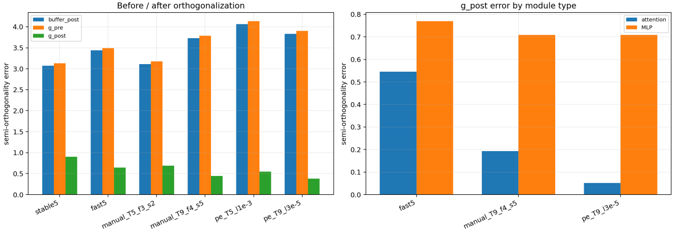
Figure 2: Spectral diagnostics from sampled update matrices. Left: error before and after the NS map. Right: module-level \mathbf{g\_post} error for representative schedules.
