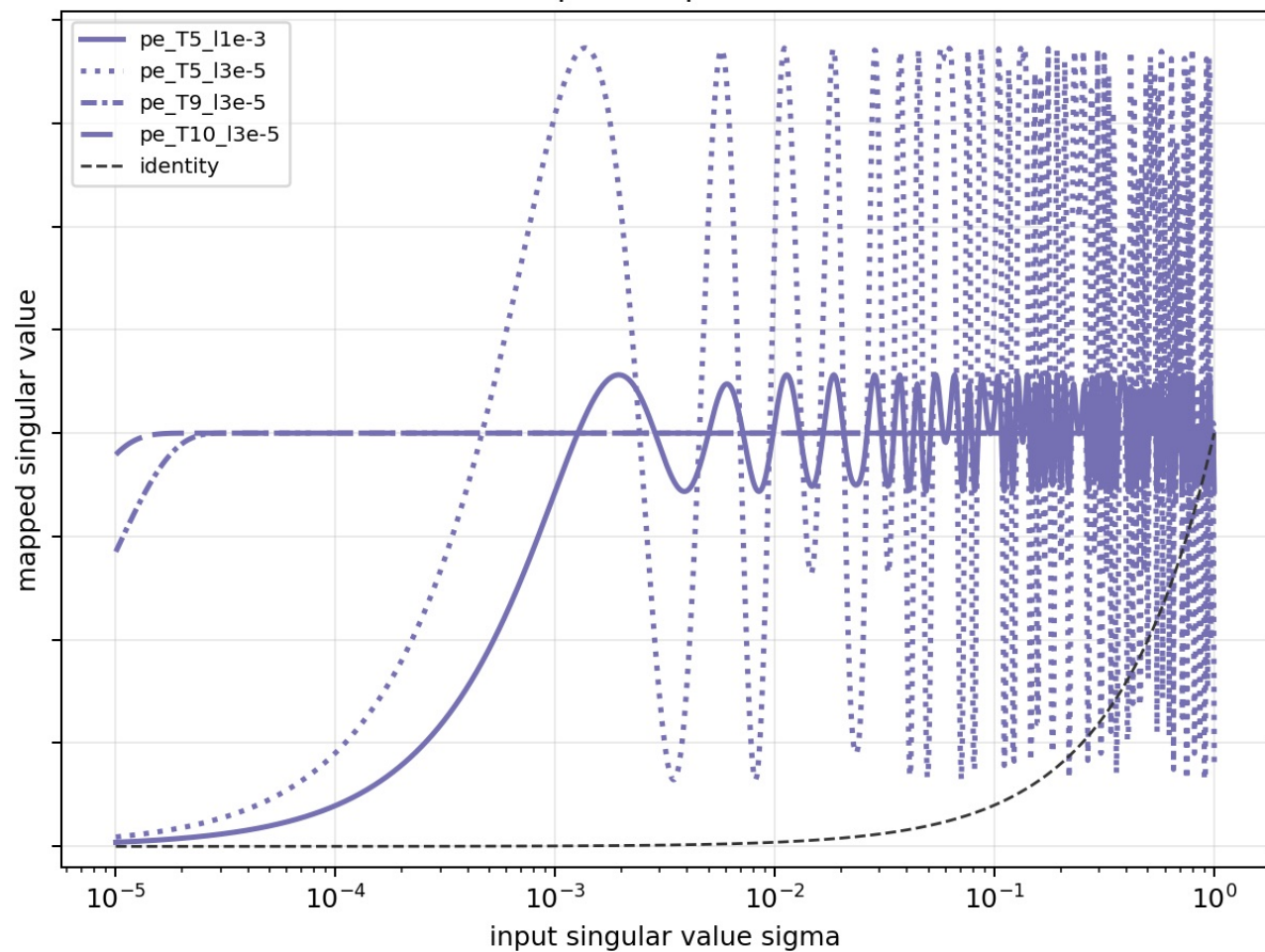
Polar Express representatives
