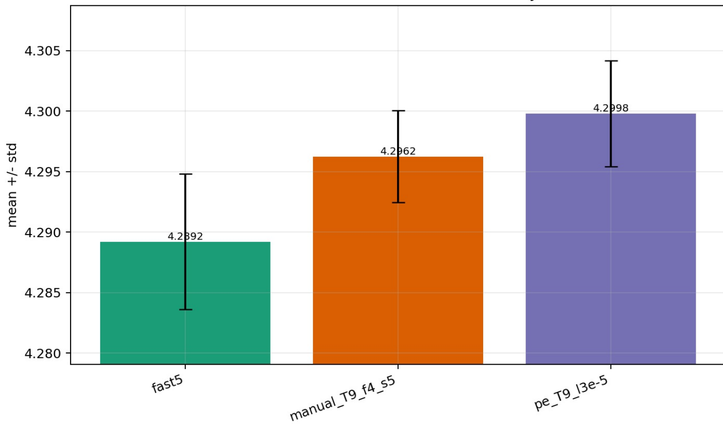
Multi-seed final validation loss (zoomed y-axis)
