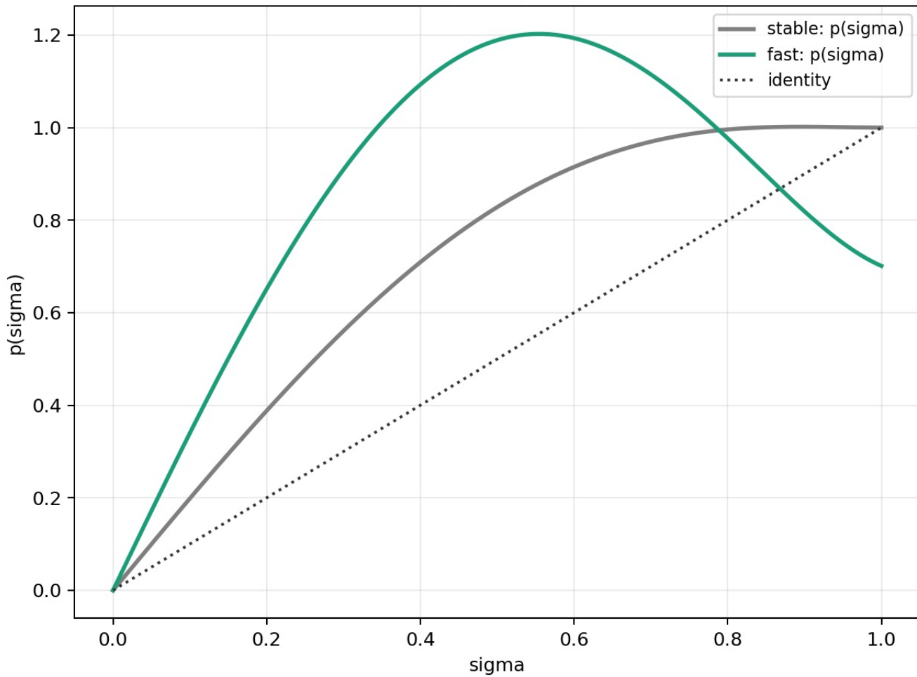
Single-step map
