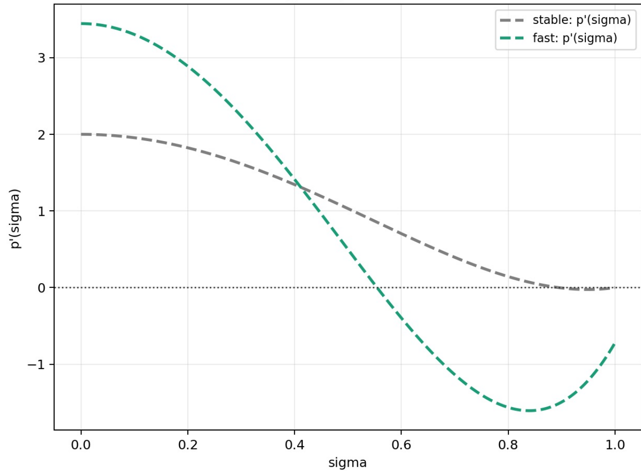
Single-step derivative
